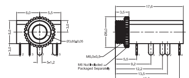
STX-3081-5C One Single Throw, Double Pole Switch
