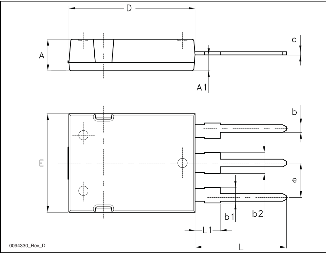
Figure 20. Max247 drawing
