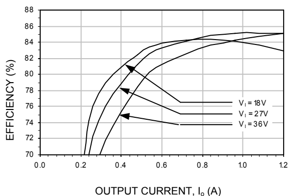
Figure 25. Converter Efficiency Vs Load.
