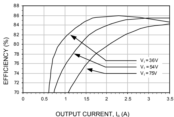
Figure 19. Converter Efficiency Vs Load.
