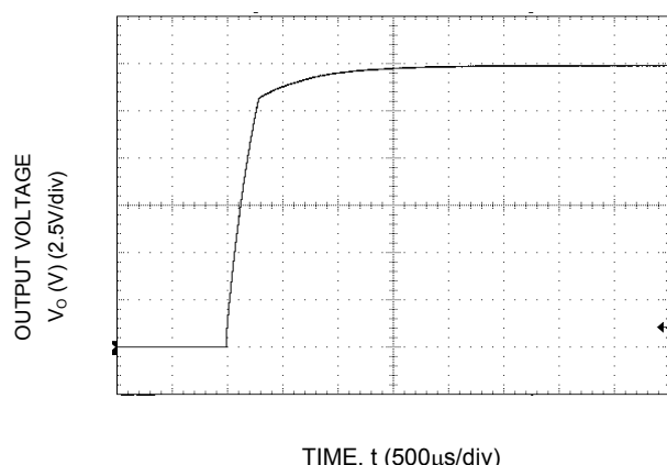
Figure 6. Typical Start-Up Output Voltage Rise Characteristic.
