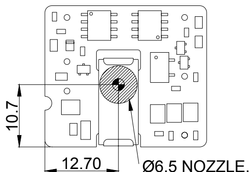
Figure 52. Pick and Place Location.
