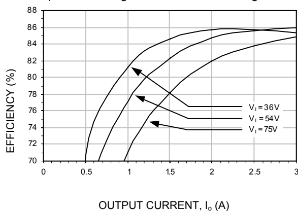
Figure 13. Converter Efficiency Vs Load at V_o = 5V .
