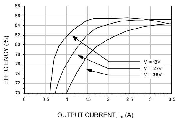
Figure 37. Converter Efficiency Vs Load.
