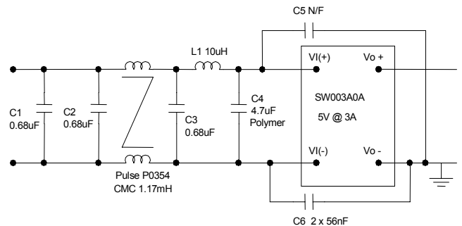
Figure 50. Suggested Configuration for EN55022 Class B.
