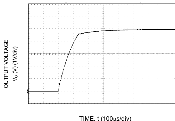
Figure 18. Typical Start-Up Output Voltage Rise Characteristic.
