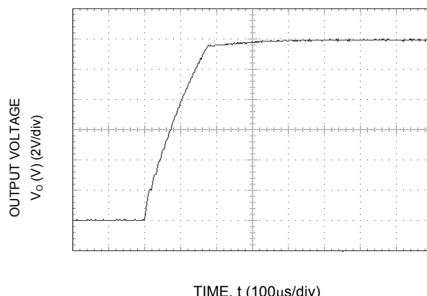
Figure 12. Typical Start-Up Output Voltage Rise Characteristic.
