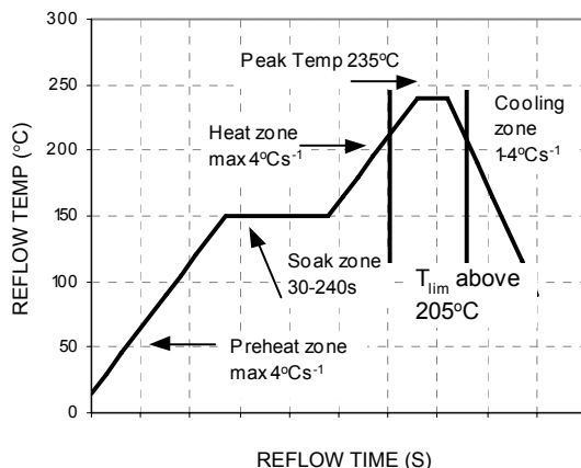
Figure 54. Recommended Reflow Profile.
