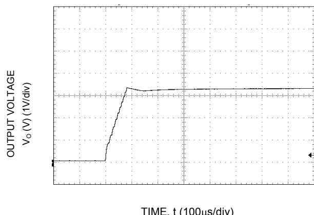
Figure 24. Typical Start-Up Output Voltage Rise Characteristic.
