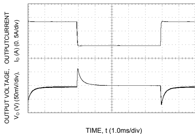
Figure 41. Transient Response to Dynamic Load Change from 50% to 75% to 50% of full load.
