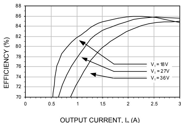
Figure 31. Converter Efficiency Vs Load.
