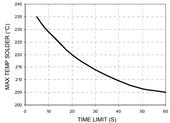
Figure 55. Time Limit Curve Above 205°C Reflow .
