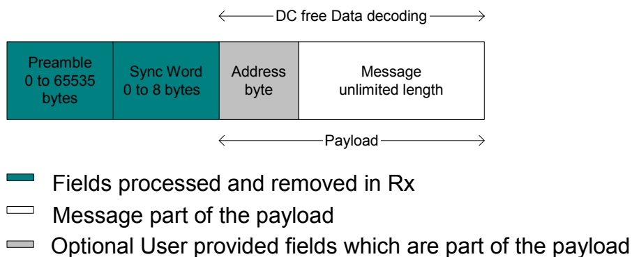
Figure 31. Unlimited Length Packet Format
