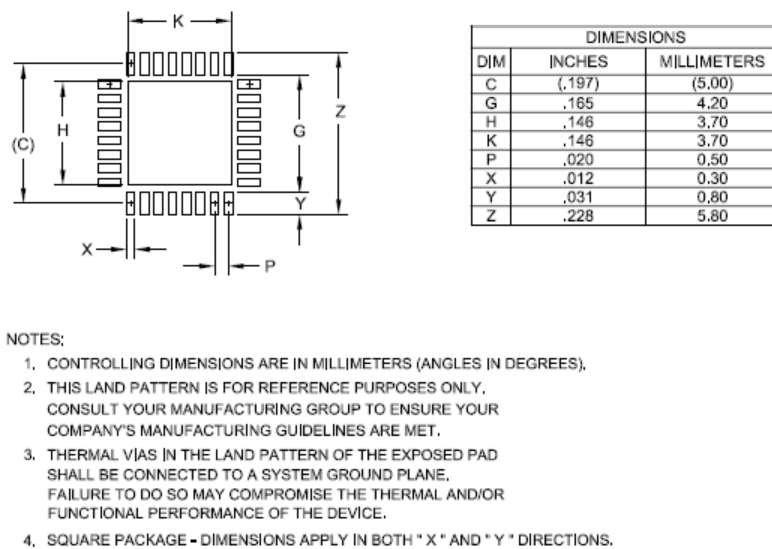
Figure 60 Land Pattern
