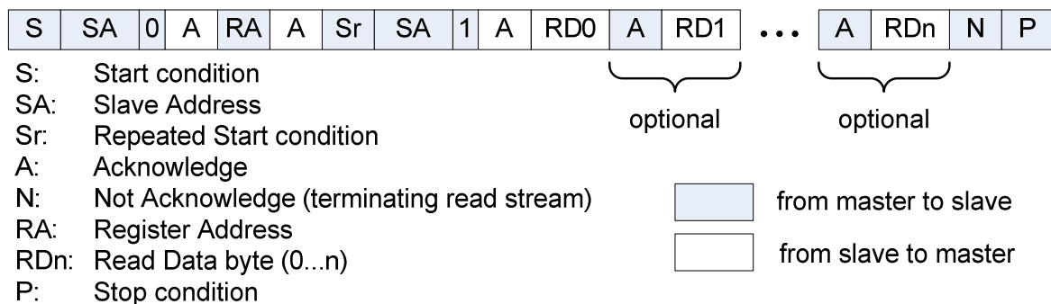
Figure 53 I2C read
