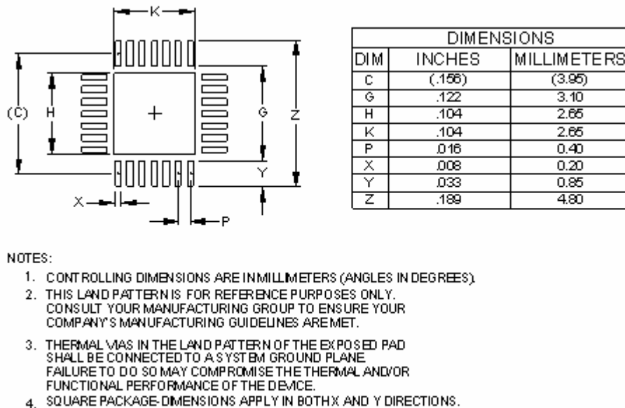
Figure 60 Land Pattern
