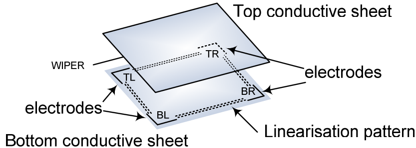
Figure 9 – 5-wire Touchscreen
