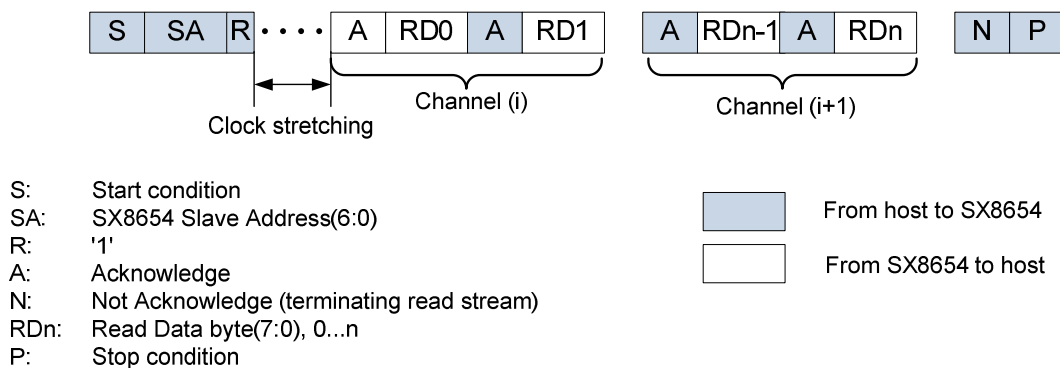
Figure 54 – I2C Read Channel
