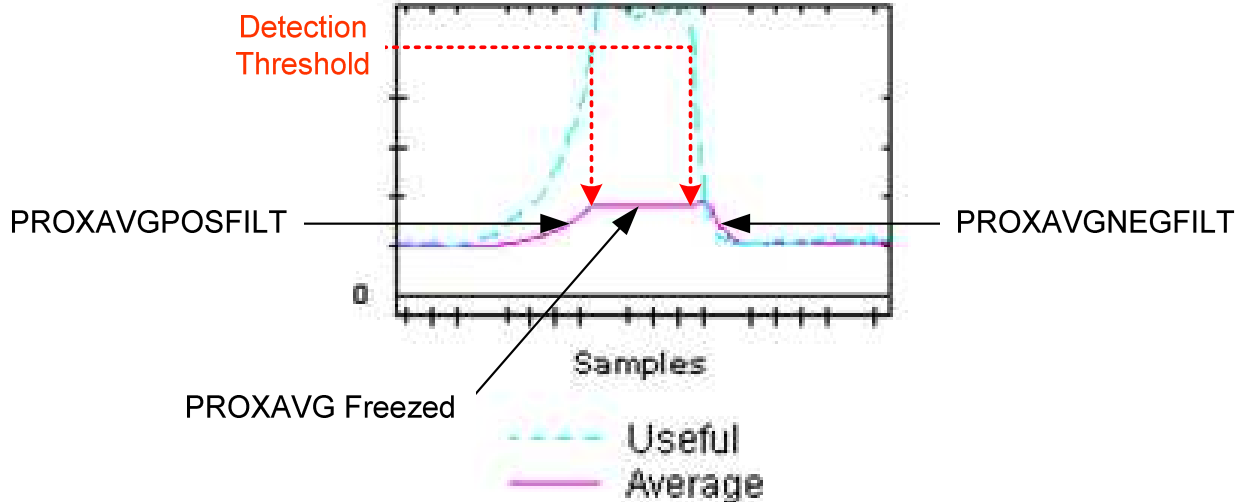
Figure 36 – ProxAvg vs Proximity Event
