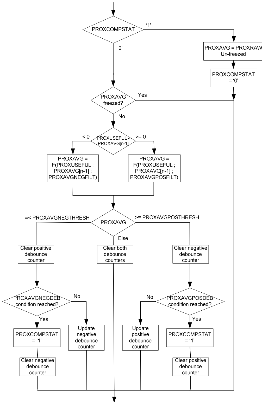
Figure 37 – ProxAvg Update
