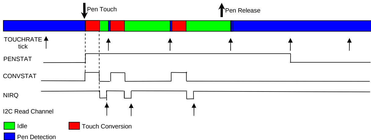
Figure 22 – Pen Trigger Mode ( \text{RegIrqMsk}[3:2] = 10 ; \text{PROXSCANPERIOD} = 0 )
