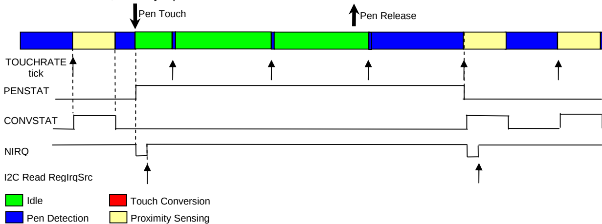
Figure 44 – Pen Detect Mode (RegIrqMsk[6:2] = 00011 ; PROXSCANPERIOD = 001 ie 1/TOUCHRATE)
