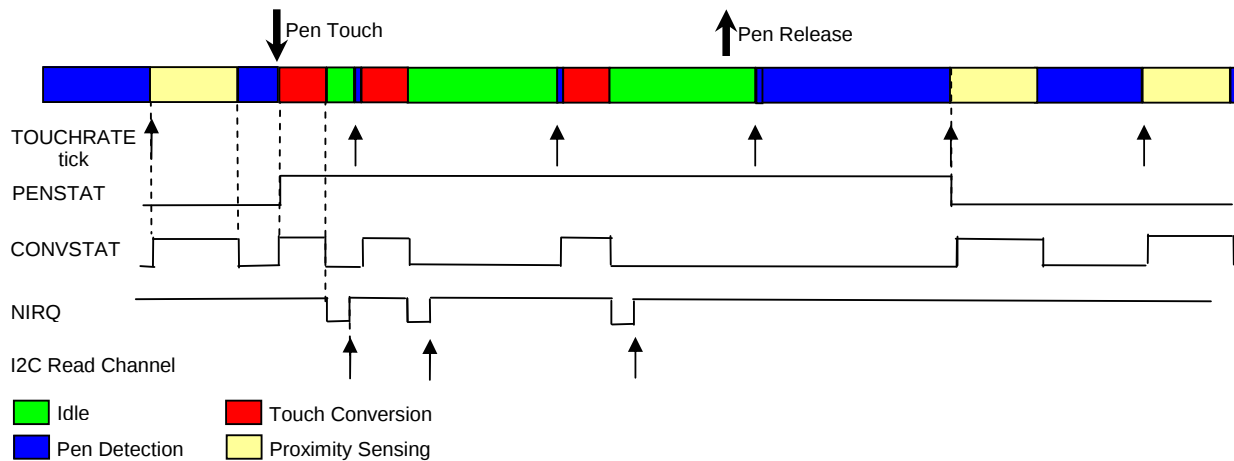
Figure 45 – Pen Trigger Mode (RegIrqMsk[6:2] = 00010 ; PROXSCANPERIOD = 001 ie 1/TOUCHRATE)
