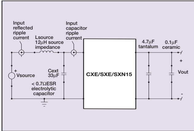
Figure 28 - Reflected Ripple Current Measurement Set-up
