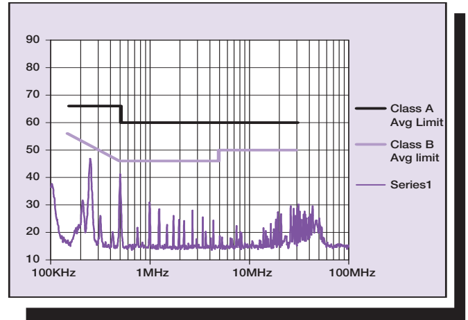
Figure 3 - SXE15-48S3V3J Conducted Noise with Recommended Class B External Filter
