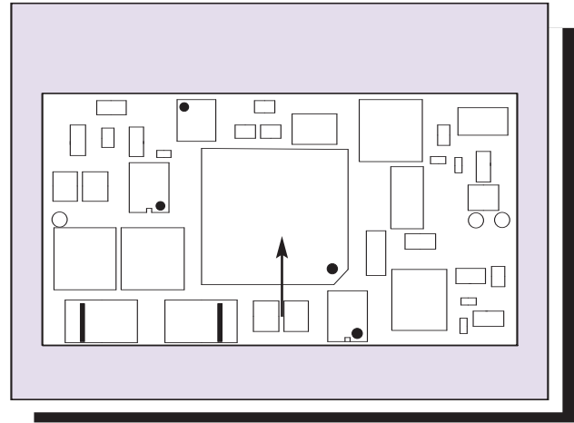
Figure 16 - Hot Spot Location on SXN15 Single
