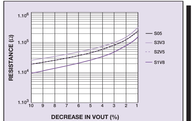
Figure 22 - Trim Up Resistance vs. Percentage Change in Output Voltage (Single Models not including SXE15-48S12J)
