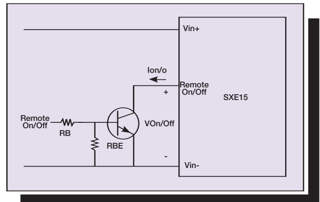
Figure 17 - Isolated Closure using a Transistor
