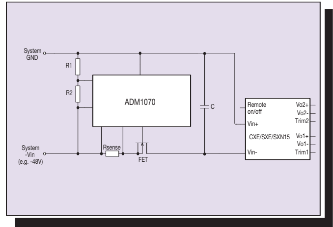
Figure 29 - Inrush Current Control Using ADM1070
