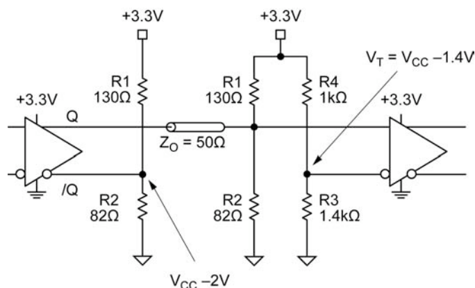
Figure 4. Terminating Unused I/O
