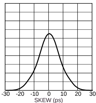
Channel-to-Channel Skew Histogram
