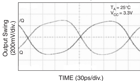
4GHz Output
