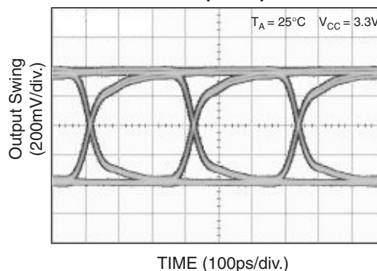
3.2Gbps Output
