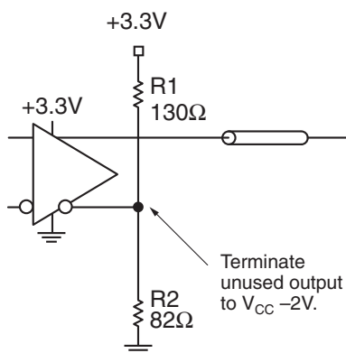
Figure 4c. Terminating Unused Outputs
