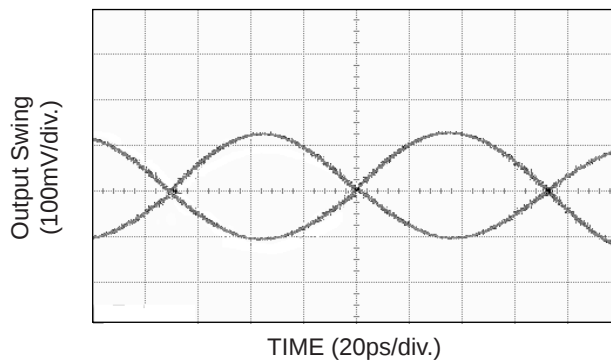
7GHz Output
