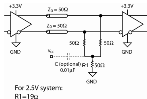
Figure 5b. Three-Resistor "Y-Termination"
