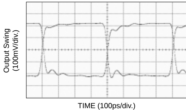
622MHz Output
