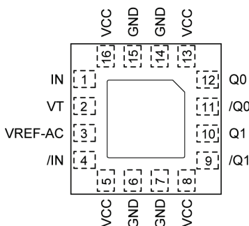
16-Pin QFN
