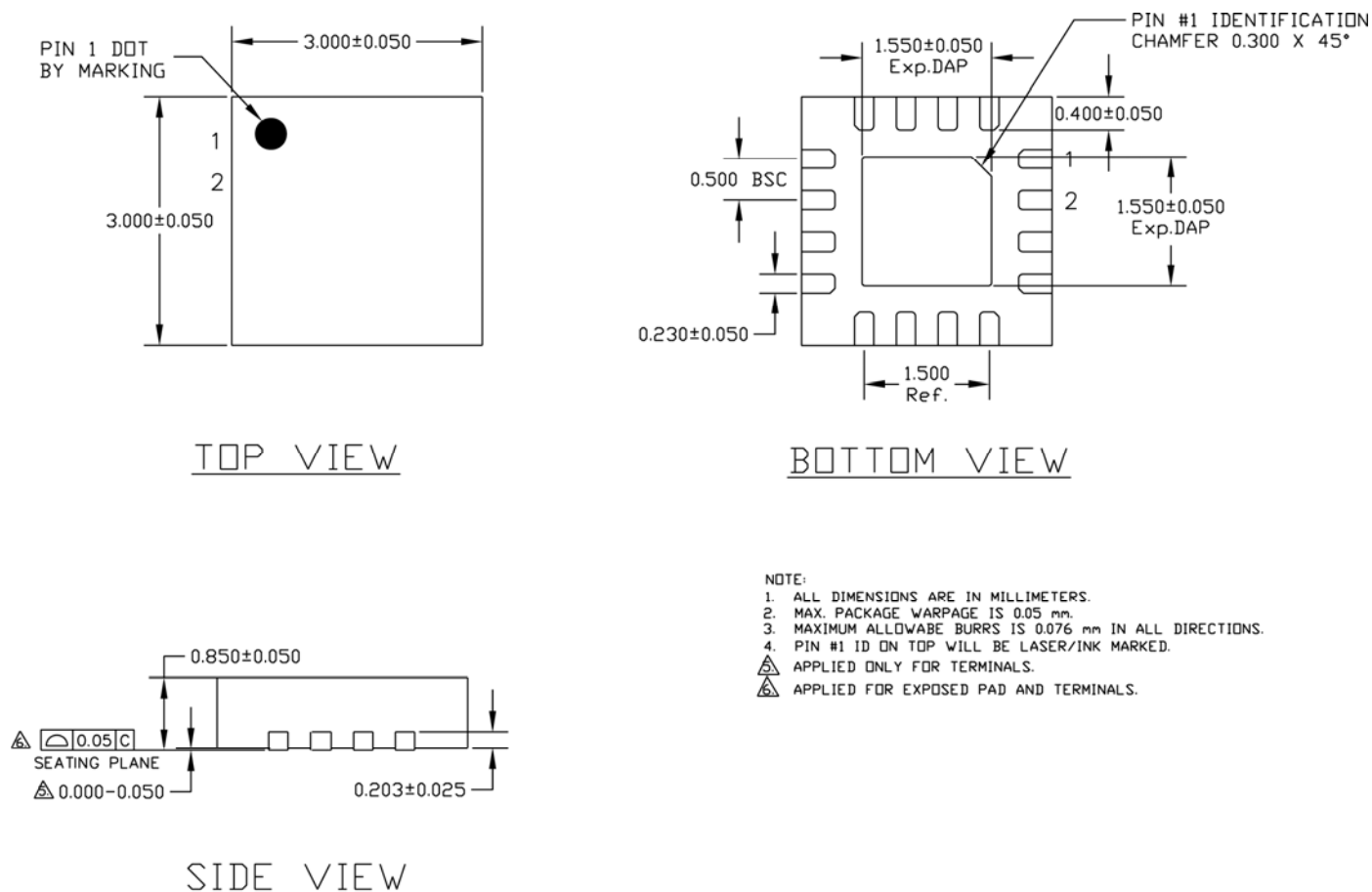
16-Pin MLF ® (3mm x3mm) (MLF-16)
