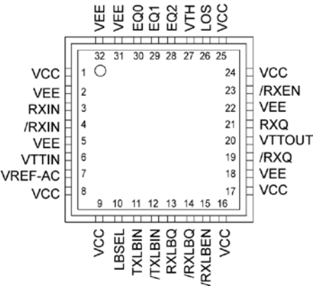
32-Pin QFN
