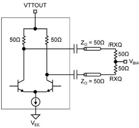
Figure 7c. CML AC-Coupled Termination
