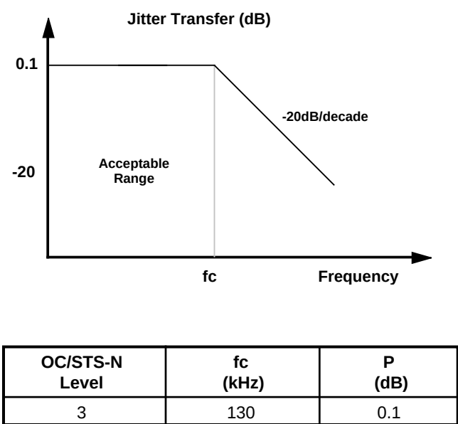
Figure 2. Jitter Transfer
