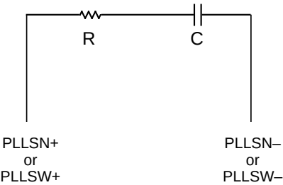
Figure 1. Narrow Band and Wide Band Synthesizer Loop Filter
