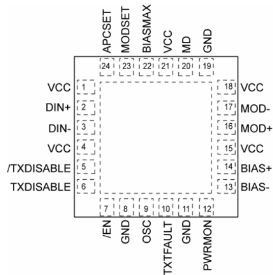
24-Pin MLF ® (MLF-24)
