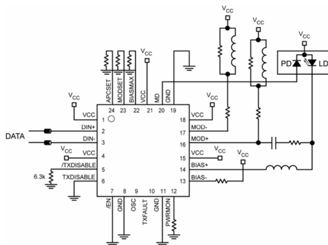
Figure 1. Laser AC-Coupled to the Driver Typical Application
