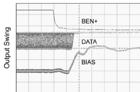
Modulation and Bias Turn-Off
