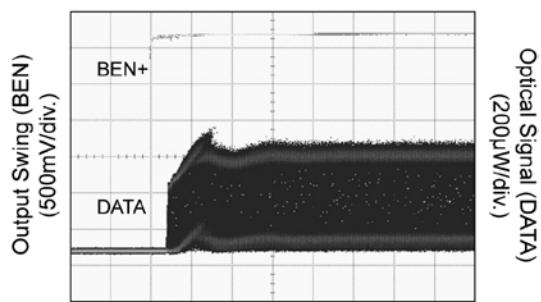
Laser Turn-On
