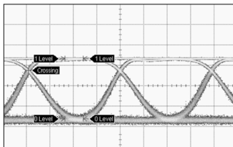
80% Crossing Point V_{THP} = 1.185V , V_{THN} = V_{THREF}
