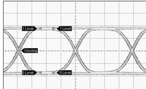
50% Crossing Point V_{THP} = 1.25V , V_{THN} = V_{THREF}
