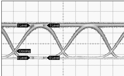
20% Crossing Point V_{THP} = 1.32V , V_{THN} = V_{THREF}
