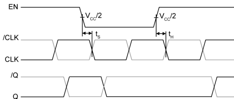
Figure 5. t_{PD} – Set-Up and Hold Time \text{EN} -to-Differential Out
