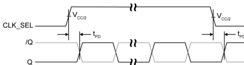
Figure 4. t_{PD} – \text{CLK\_SEL} -to-Differential Out
