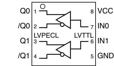
8-Pin MLF® Ultra-Small Outline (2mm × 2mm)
