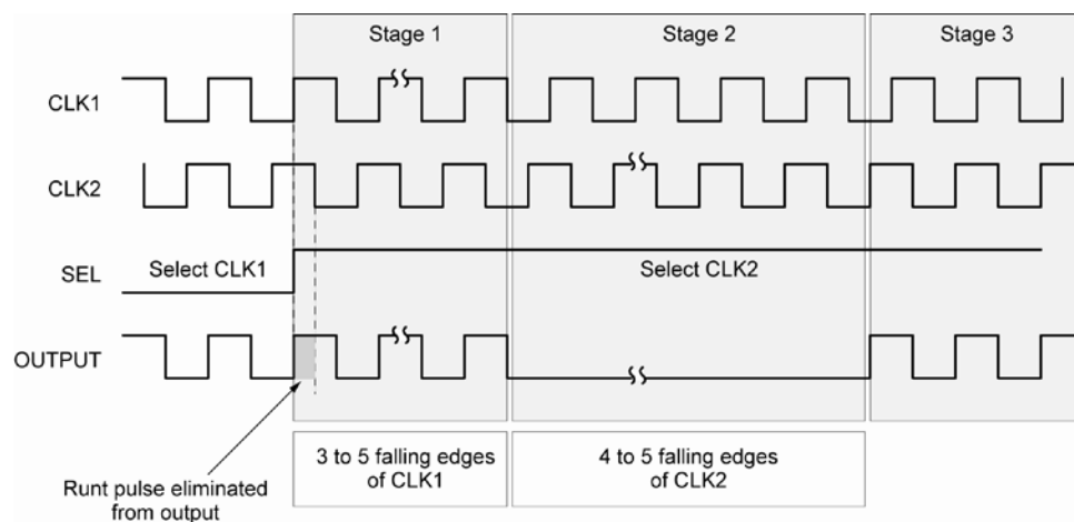
Timing Diagram 1
