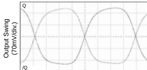
1.6GHz Output
