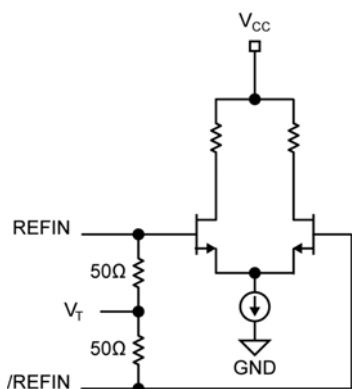
Figure 1a. Simplified Differential Input Buffer
