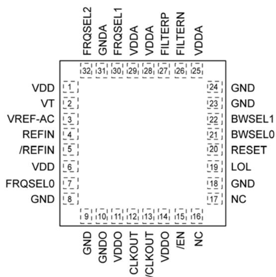
32-Pin QFN
