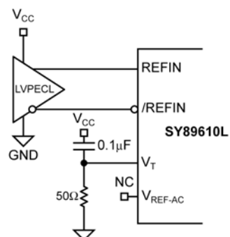
Figure 3c. LVPECL Interface (DC-Coupled)
