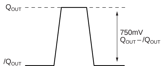
Figure 6. Output Driver Signal Levels (Differential)
