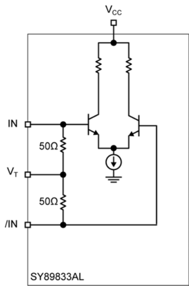
Figure 1. Simplified Differential Input Buffer
