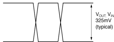
Figure 2c. Single-Ended Swing
