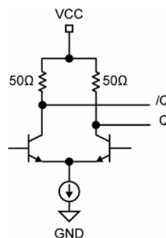
Figure 2b. Simplified Differential Output Stage
