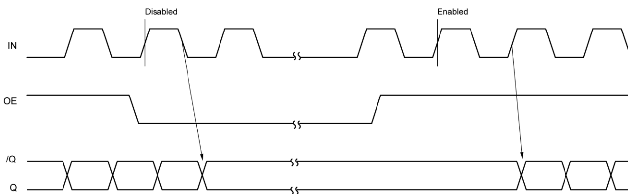
Figure 1b. Enable Output Timing Diagram
