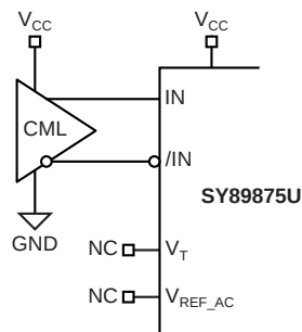
Figure 4a. DC-Coupled CML Input Interface
