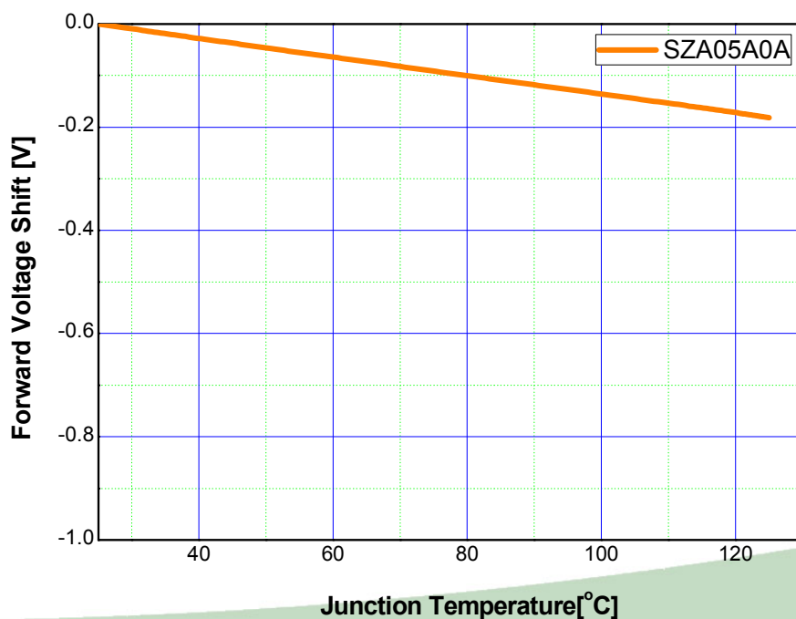
Junction Temperature vs. Forward Voltage at I_F=350\text{mA}
