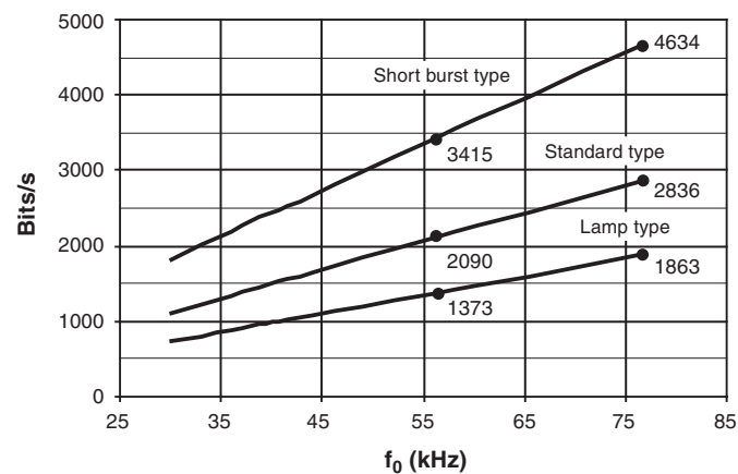
Figure 6-3. Data Transmission Rate, V_S = 5V
