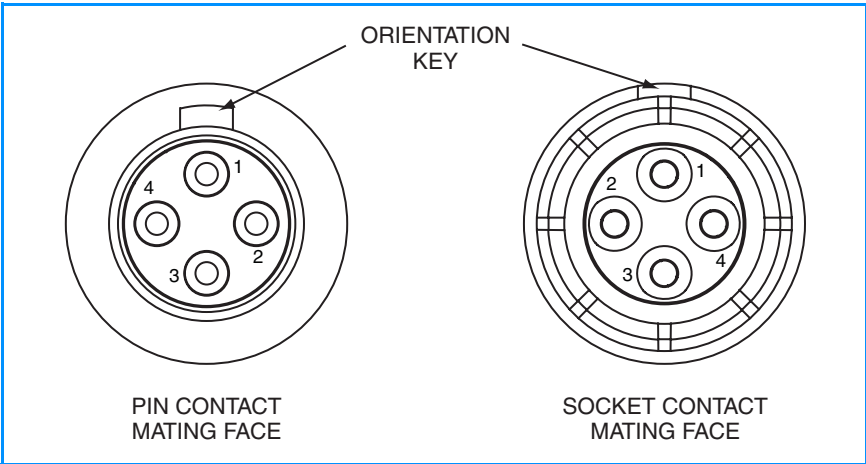
FIGURE 1 - INNER CONTACT NUMBERING, QUADRIX
