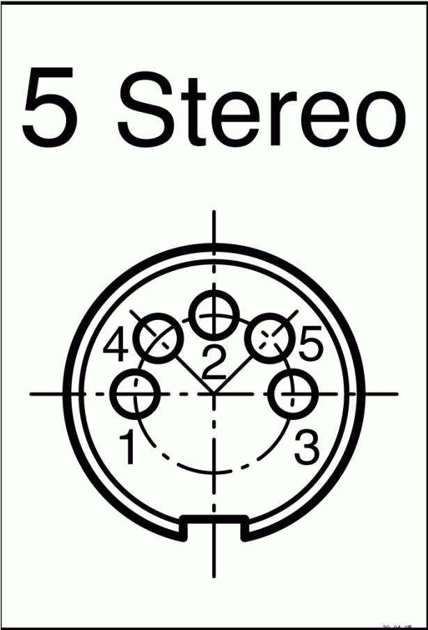
Contact arrangement
