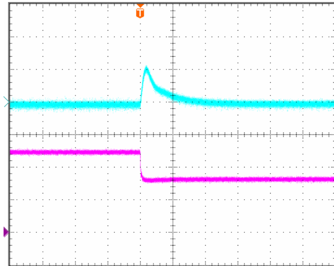
Figure 8: Output voltage response to step-change in load current (75%-50% of I_o , max; di/dt = 1A/\mu s ). Load cap: 400\mu F , ceramic capacitor. Top Trace: V_{out} (100mV/div, 200us/div); Bottom Trace: output current (1.5A/div, 200us/div)
