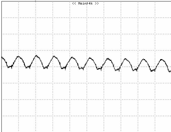
Figure 12: Input reflected ripple current, i_s , through a 12\mu\text{H} source inductor at nominal input voltage and rated load current ( 20\text{ mV/div} , 2\mu\text{s/div} ). Setup is shown in Figure 10 top picture.
