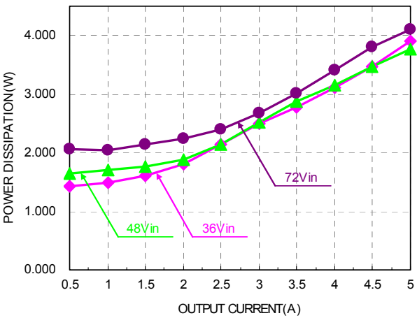
Figure 2: Power dissipation vs. load current for minimum, nominal, and maximum input voltage.
