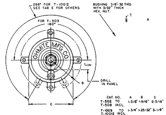
Fig. 216—Dimensions of Non-Shorting Tap Switches.
