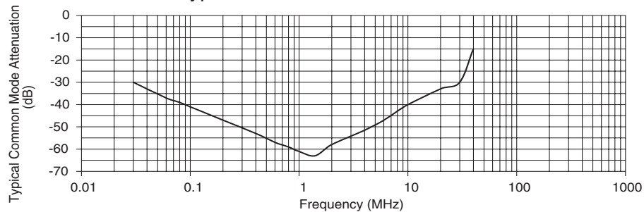
Typical Common Mode Impedance
