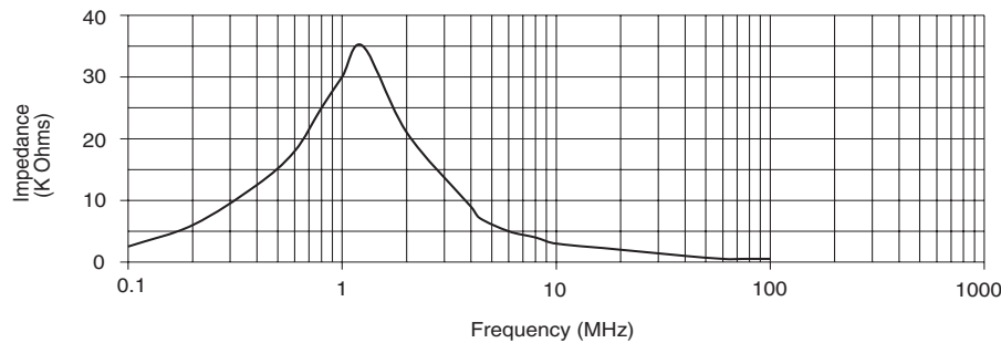
Typical Common Mode Attenuation
