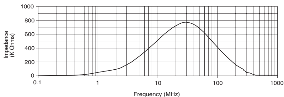
Typical Common Mode Impedance
