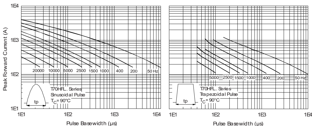
Fig. 41 - Frequency Characteristics
