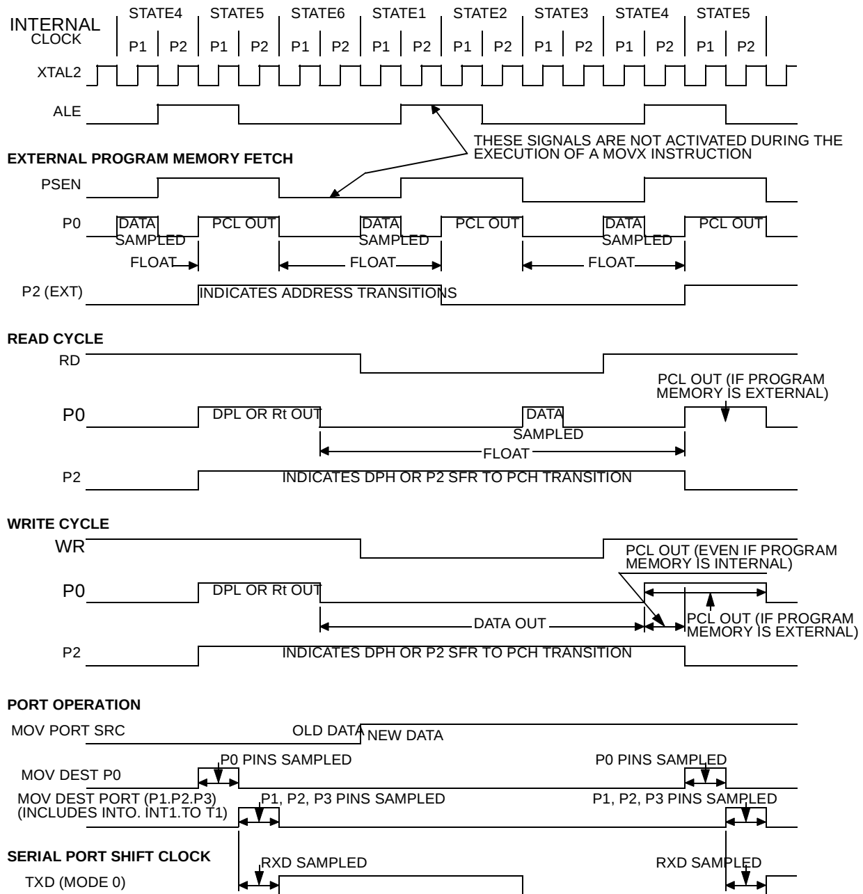
Figure 45. Clock Waveforms
