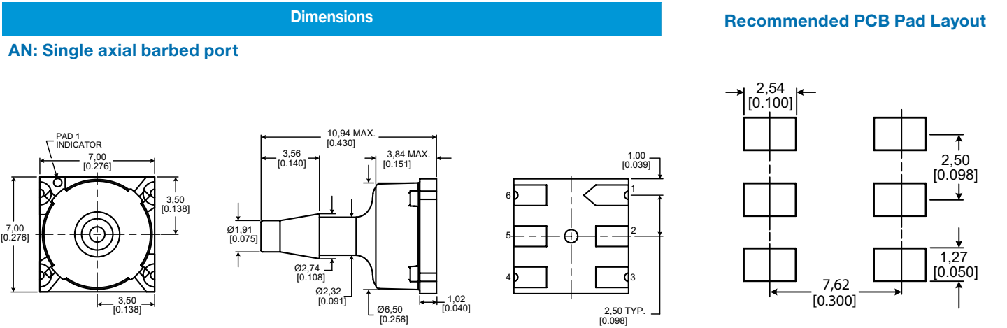
Figure 4. Leadless SMT Package Dimensional Drawings (For reference only: mm [in].)
