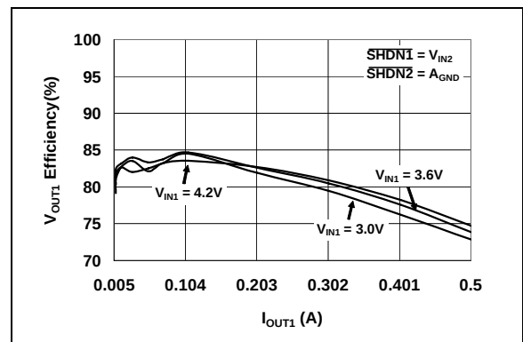
FIGURE 2-5: V_{OUT1} Output Efficiency vs. I_{OUT1} ( V_{OUT1} = 1.2\text{V} ).
