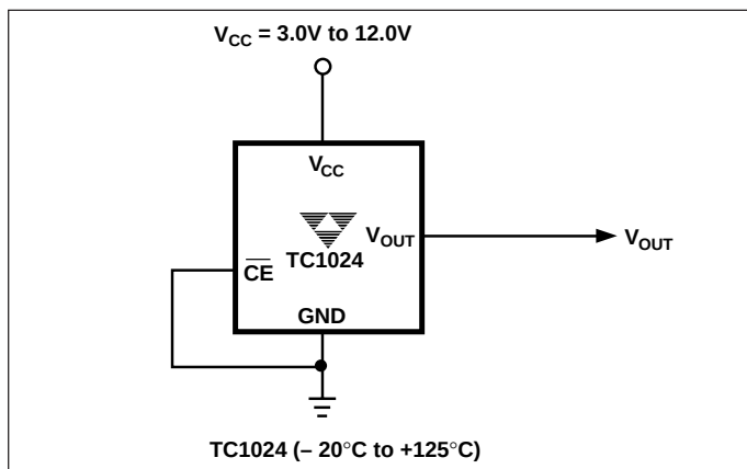
Figure 2. TC1024 Connections
