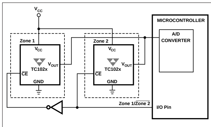
Figure 4. TC1023/1024 Addressing
