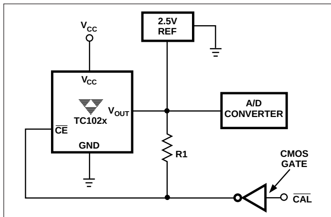
Figure 3. A/D Calibration
