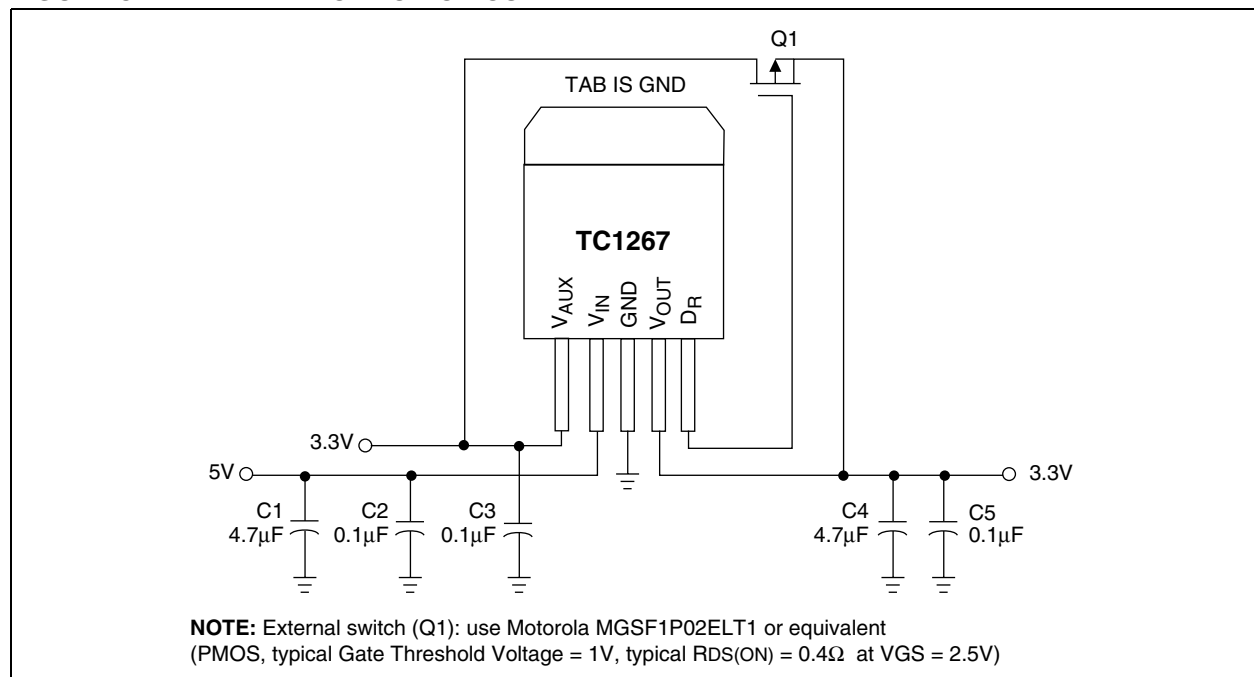
FIGURE 3-1: APPLICATION CIRCUIT
