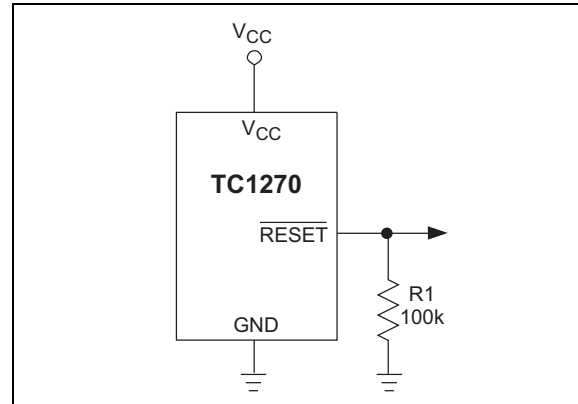
FIGURE 4-2: Ensuring \overline{\text{RESET}} Valid to V_{CC} = 0V .
