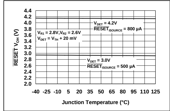
FIGURE 2-32: RESET Output Voltage High vs. Junction Temperature.
