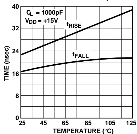
Rise and Fall Times vs. Temperature
