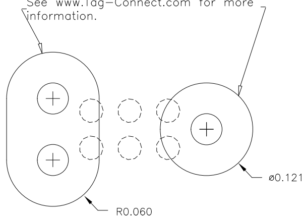
OPTIONAL BOTTOM LAYER ALTERNATIVE - USE TC2030-CLIP BOARD
