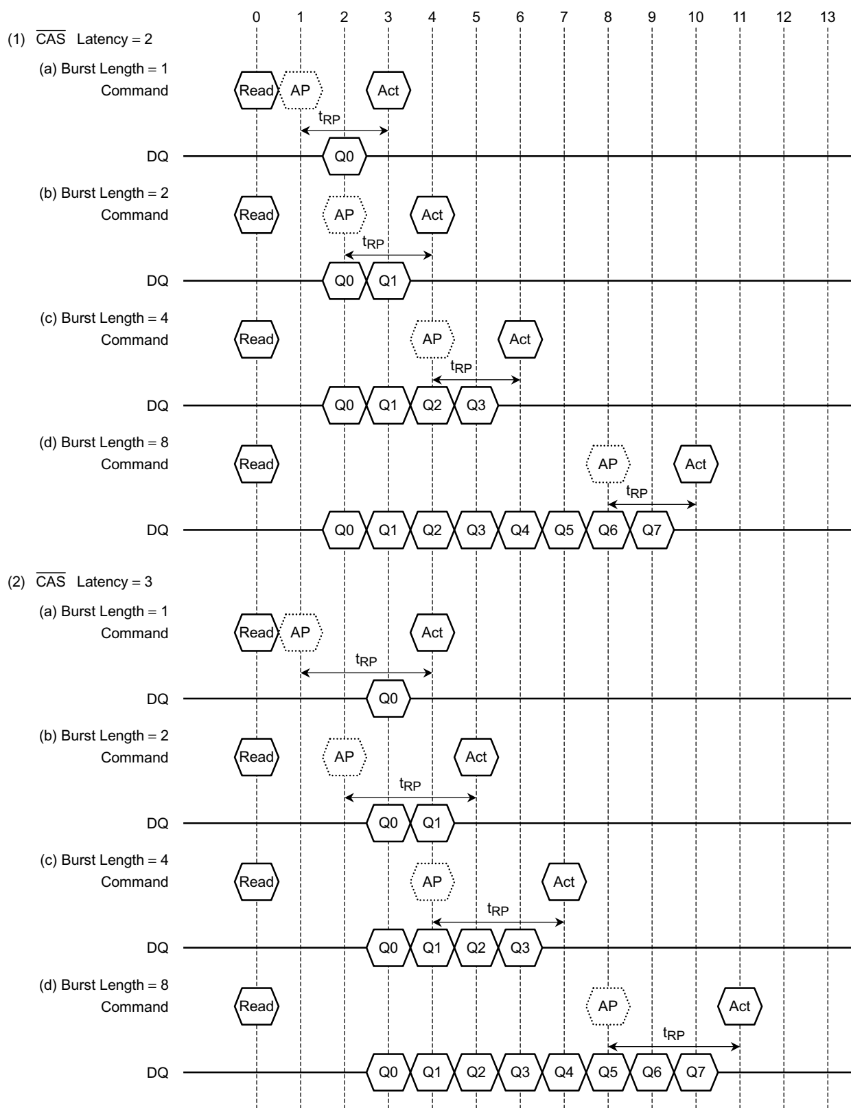
Figure 15. Auto Precharge timing (Read cycle)
