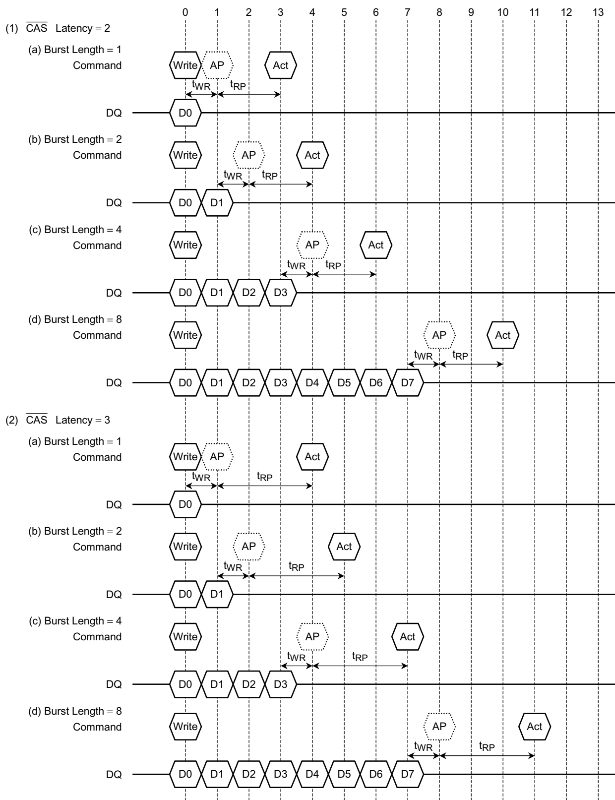
Figure 16. Auto Precharge timing (Write cycle)
